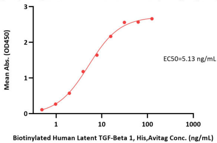
Cynomolgus ITGAV&ITGB8 Heterodimer Protein, His Tag&Tag Free ELISA 0.5 µg of Cynomolgus ITGAV&ITGB8 Heterodimer Protein, His Tag&Tag Free per well
